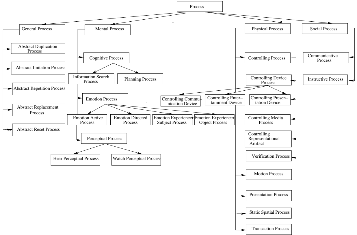
Figure 1: Upper part of the process hierarchy.
