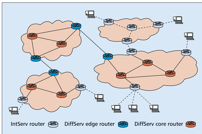
■ Figure 2. An example IntServ over DiffServ scenario.
