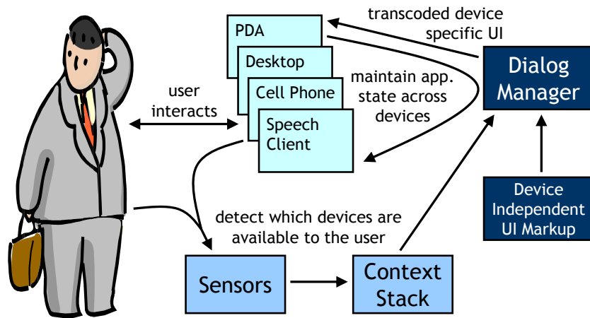
Figure 2. Architecture sketch
